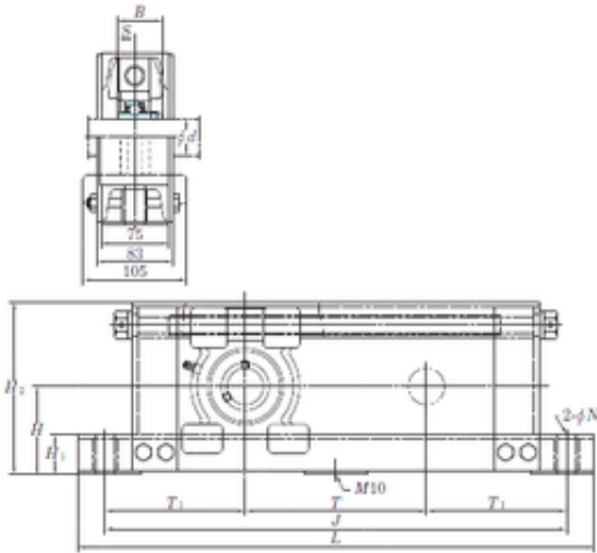
Bearing No. UCTU211-600
