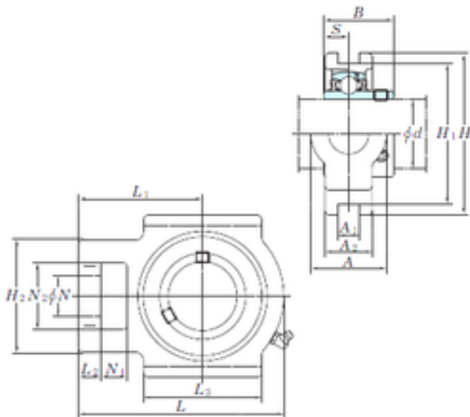
Bearing No. UCT215-48E
