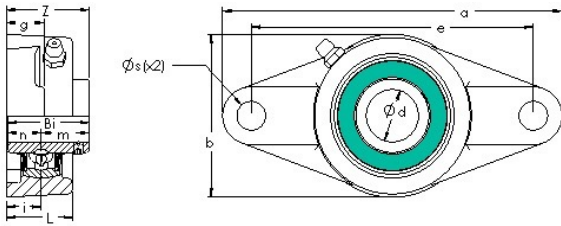
Bearing No. UCFL 205-16G5PL
